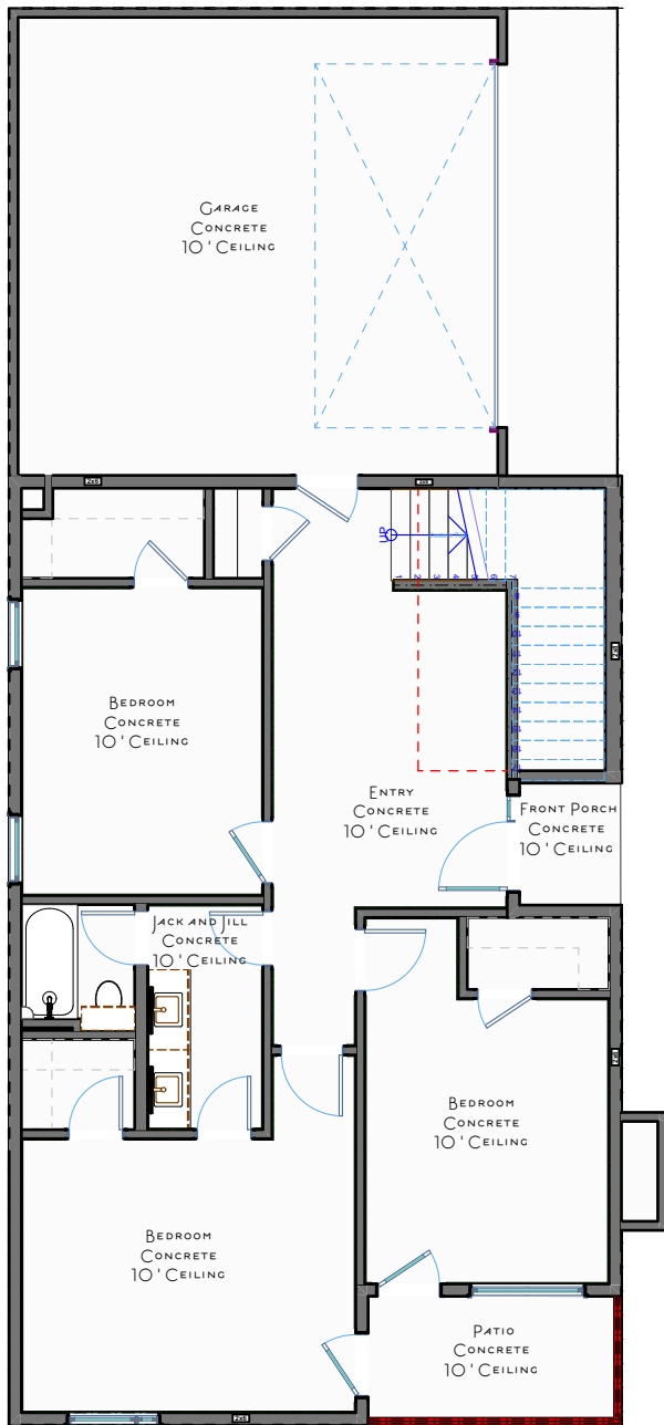
FIRST FLOOR
